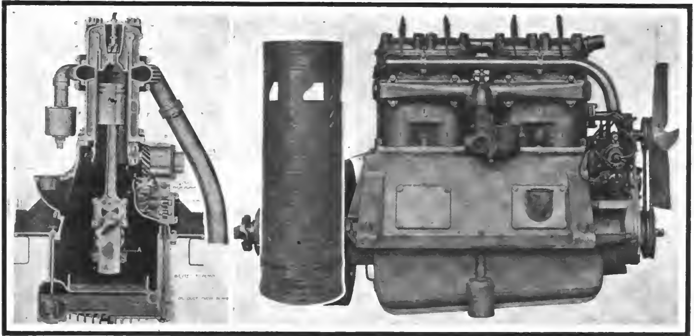
Vertical section and side view of the Argyll single-sleeve motor
